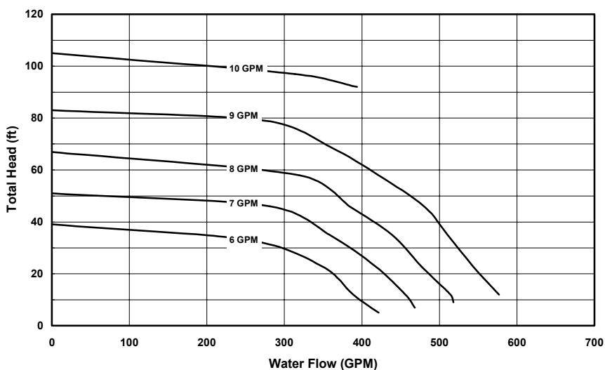
SM50 Pump Performance
